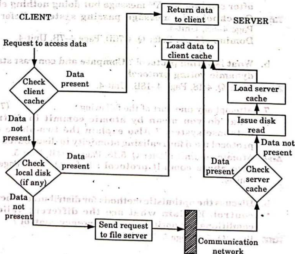
Fig. 1. Data access action in distributed file system.
