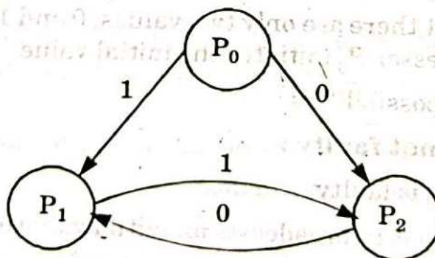
Fig. 3.8.2 Processor P_0 is faulty.
