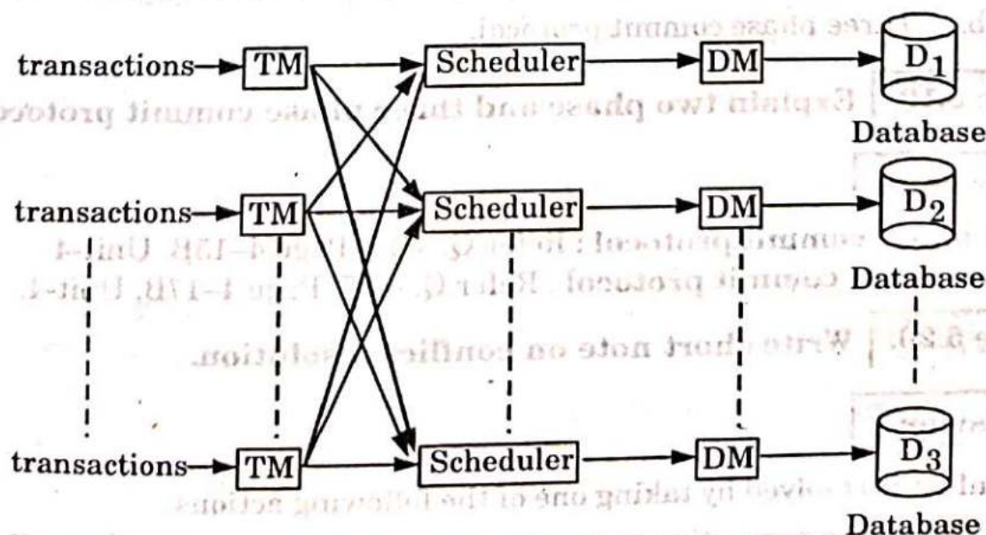
Fig. 5.17.1. Distributed transaction management model.
