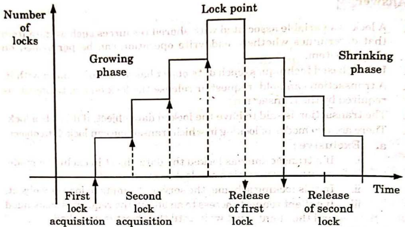
Fig. 5.5.1. Two phase locking scheme.
