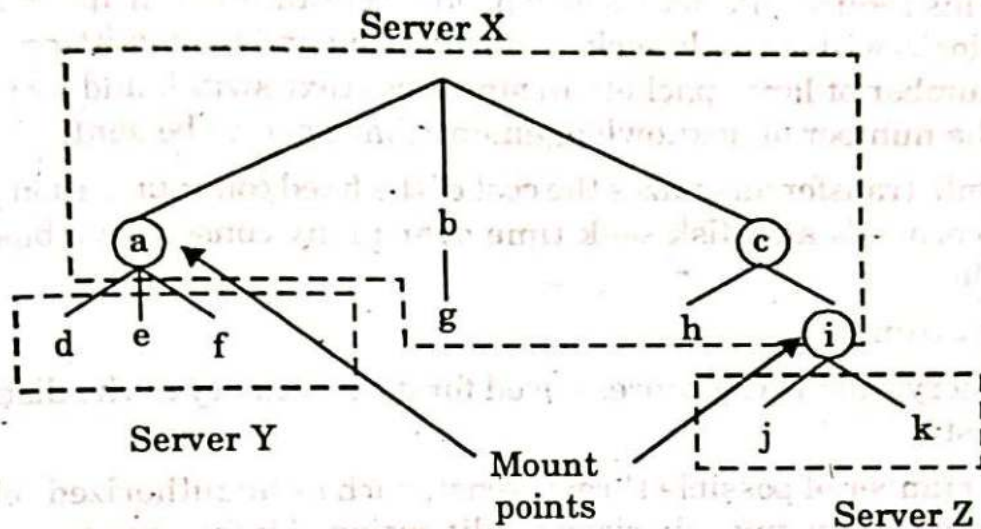
Fig. 3.16.1. Name space hierarchy.
