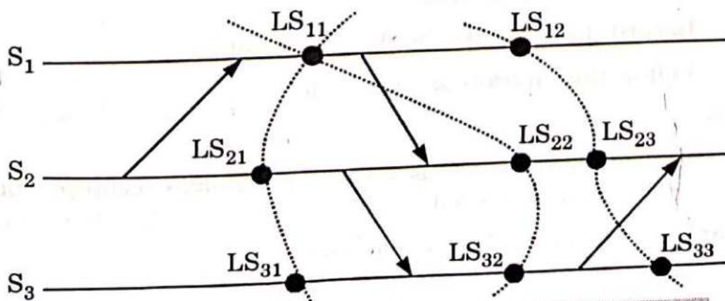
Fig. 1.17.1. Global states in a distributed computation.
