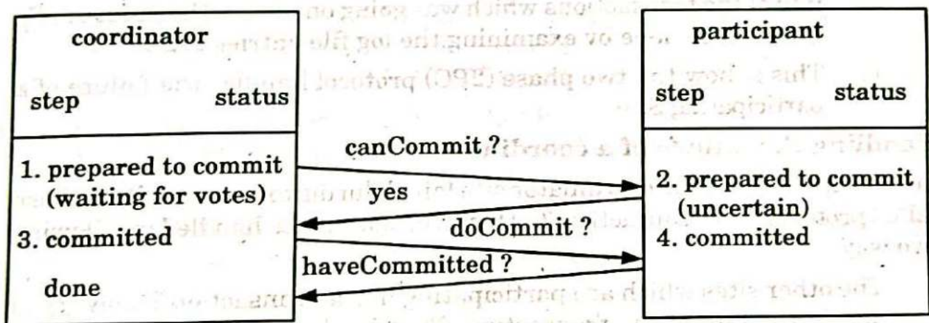
Fig. 4.15.1. Communication in two phase commit protocol.
