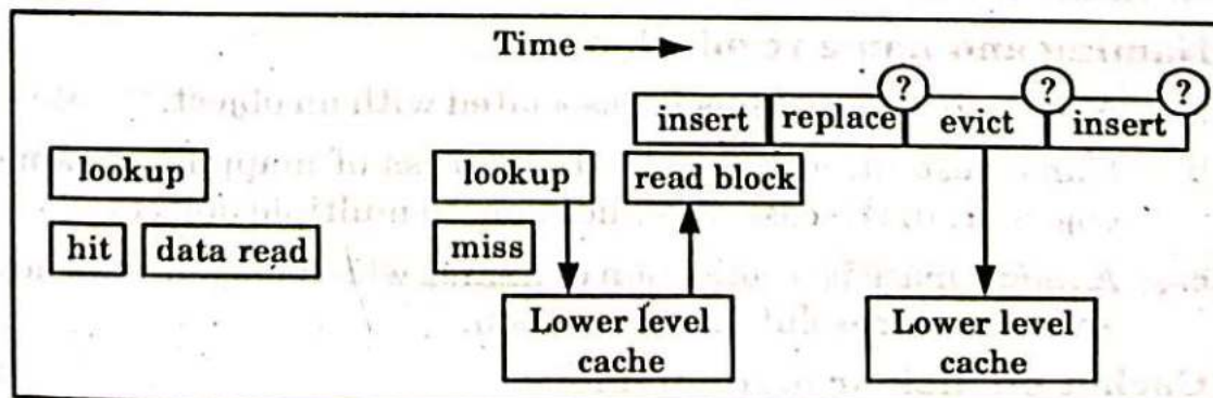
Fig. 3.18.1. The read operation.
