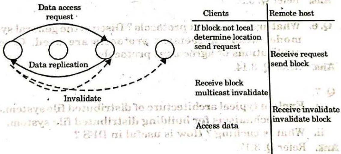
Fig. 3.29.1. Write operation in the read replication algorithm.
