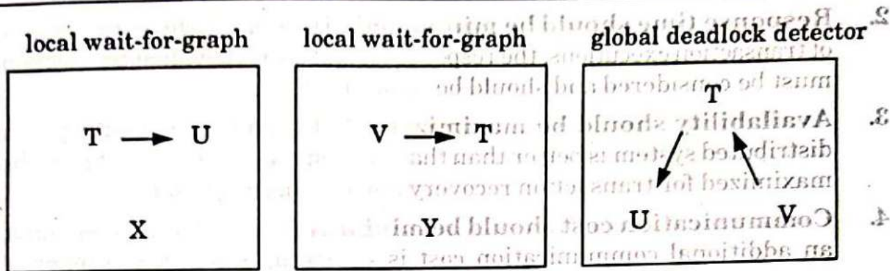
Fig. 5.26.1. Local and global wait-for-graphs.
