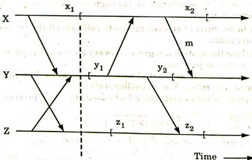
Fig. 4.4.1. Consistent set of checkpoints.
