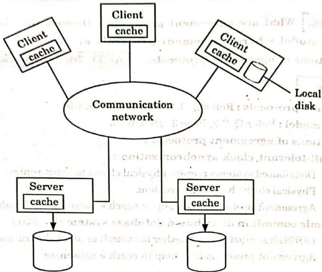
Fig. 3.15.1. Architecture of DFS.
