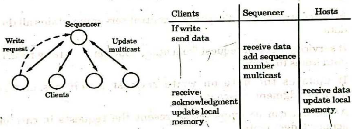
Fig. 3.26.1. Full replication algorithm.
