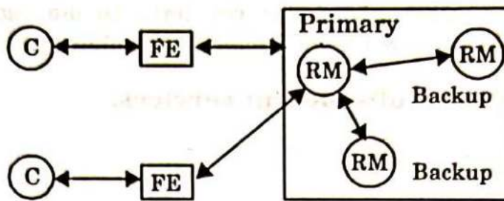
Fig. 5.35.1. The passive (primary-backup) model for fault tolerance.
