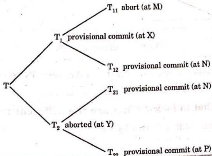
Fig. 5.3.1. Transaction T decides whether to commit.
