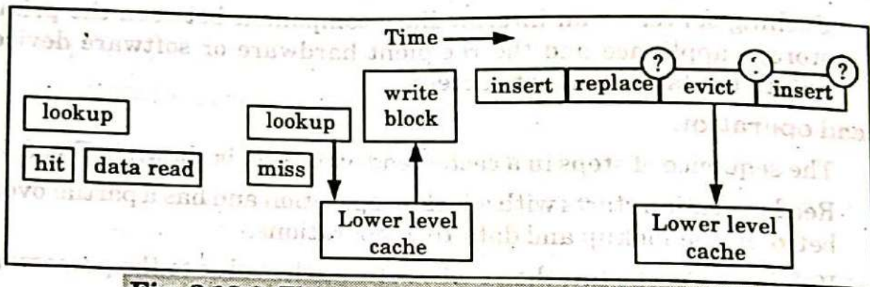
Fig. 3.18.2. The write operation (write back cache).
