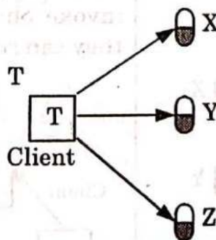
Fig. 5.15.1. Flat transactions.
