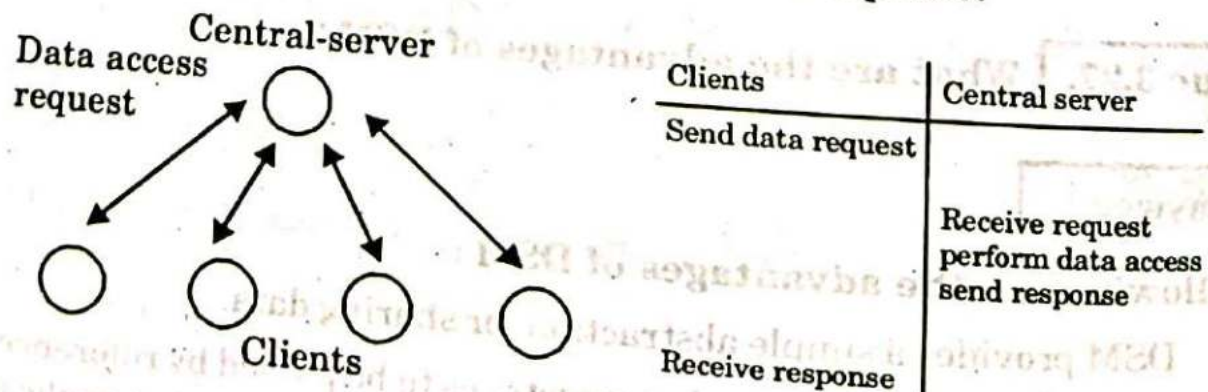
Fig. 3.28.1. Central-server algorithm.
