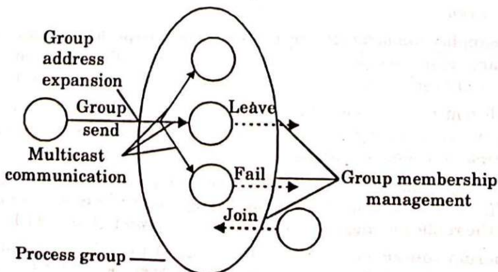
Fig. 5.34.1. Services provided for process groups.
