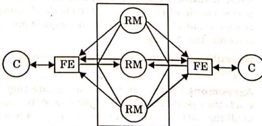
Fig. 5.35.2. Active replication.
