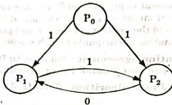
Fig. 3.8.1 Processor P_0 is non-faulty.
